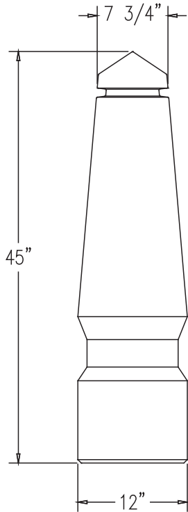
ELEVATION VIEW
