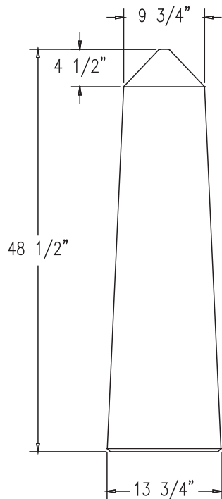
ELEVATION VIEW
