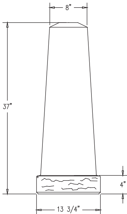
ELEVATION VIEW
