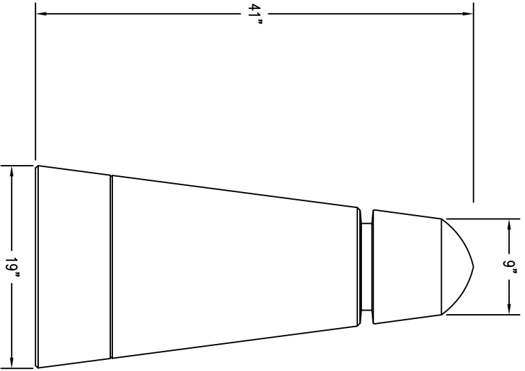
1 TOP VIEW
