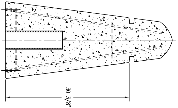
4 CROSS SECTION
