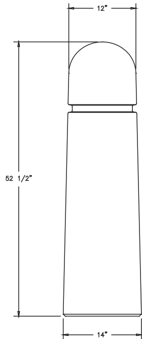
ELEVATION VIEW
