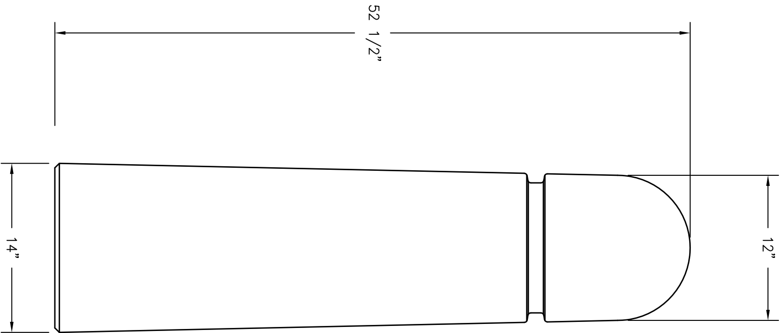
2 ELEVATION VIEW
