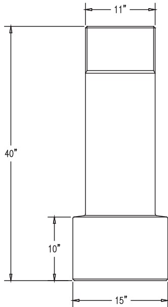
ELEVATION VIEW
