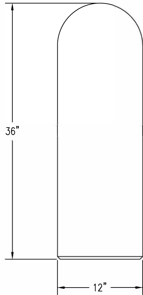
2 ELEVATION VIEW
