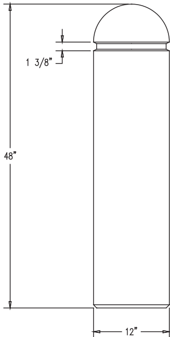
ELEVATION VIEW
