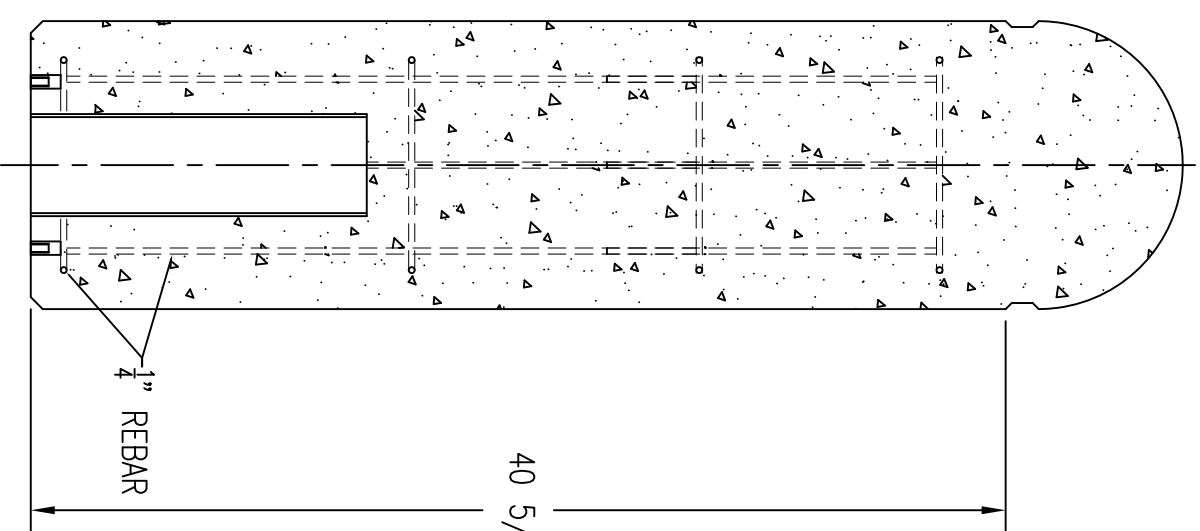
4 CROSS SECTION
