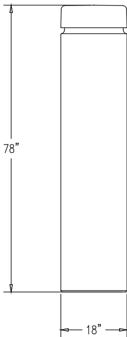
ELEVATION VIEW
