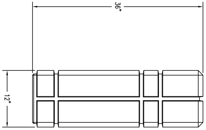
2 ELEVATION VIEW
