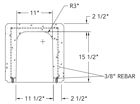
5 SECTION VIEW
