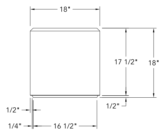
4 END VIEW
