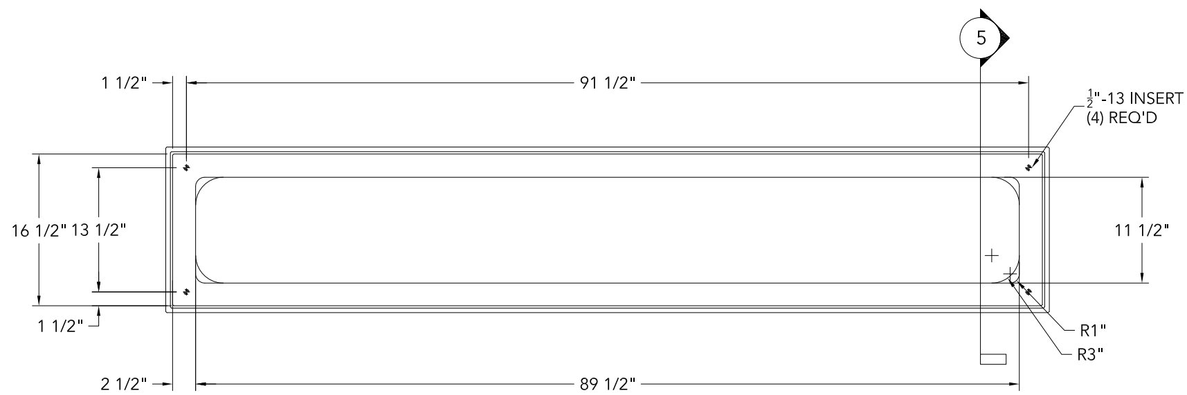
3 BOTTOM VIEW
