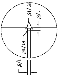
A ENLARGED DETAIL OF REVEAL LINE Scale: 1" = 1"
