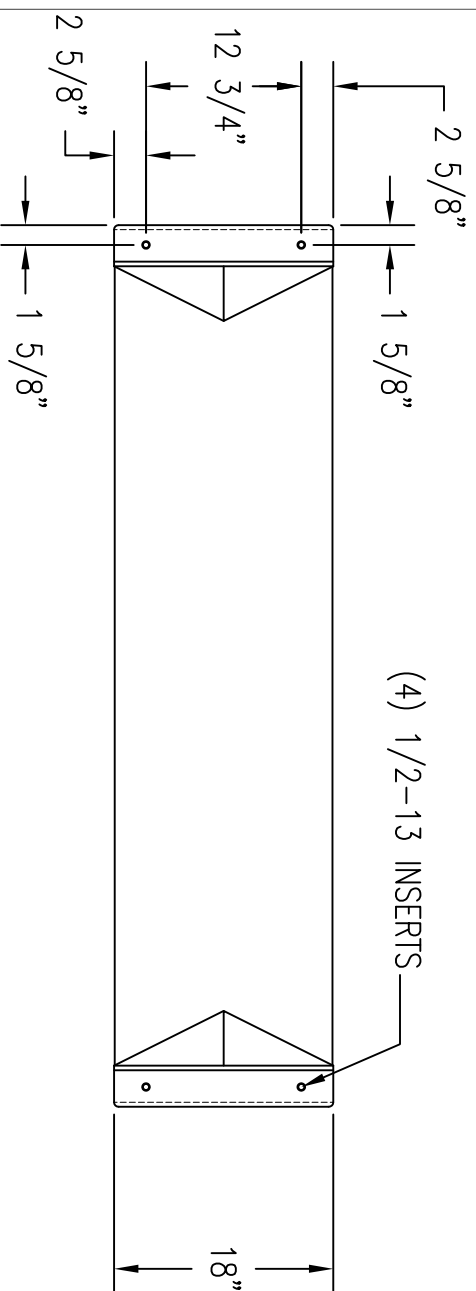
3 BOTTOM VIEW Scale: 1/16" = 1"
