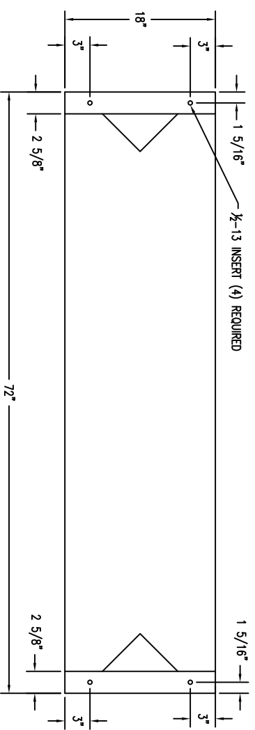
BOTTOM VIEW
