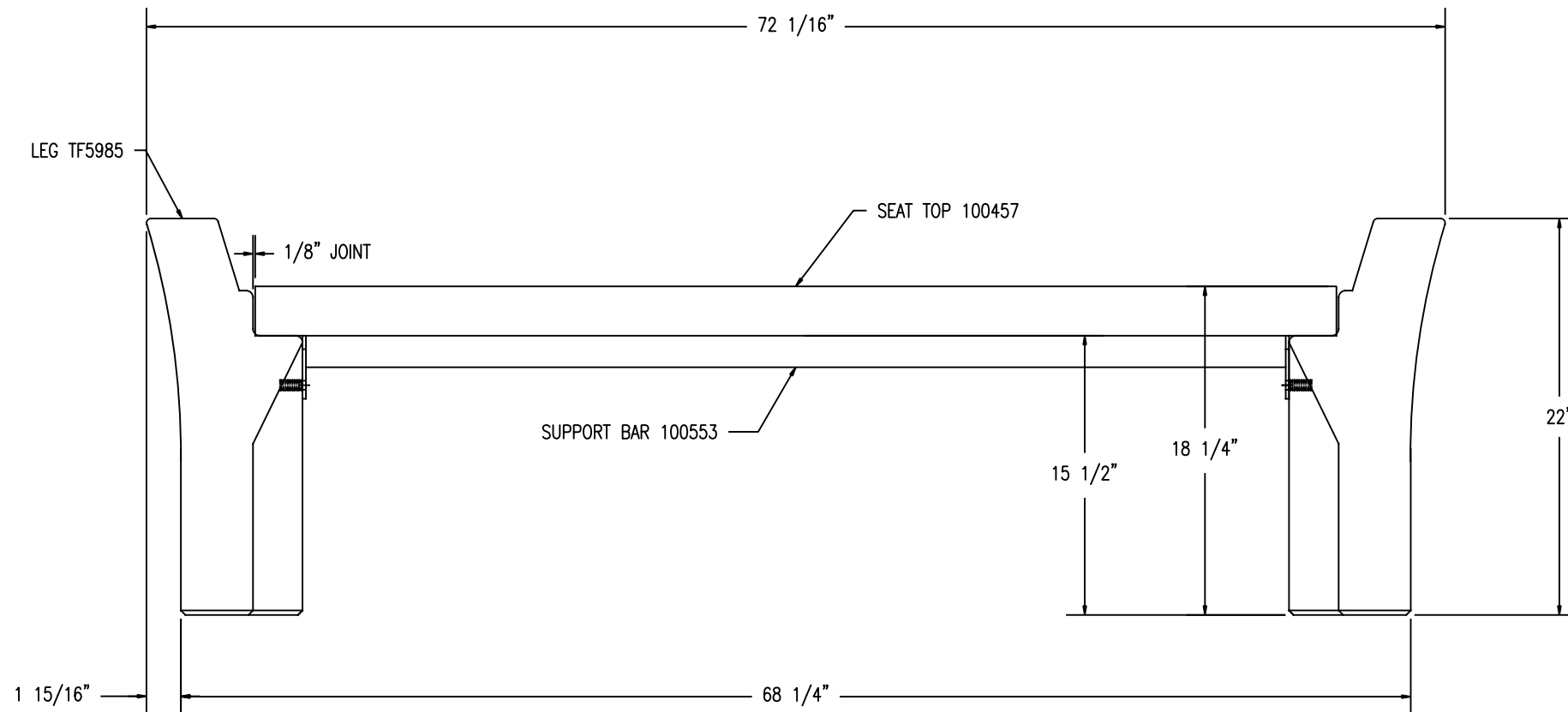
2 SIDE VIEW
