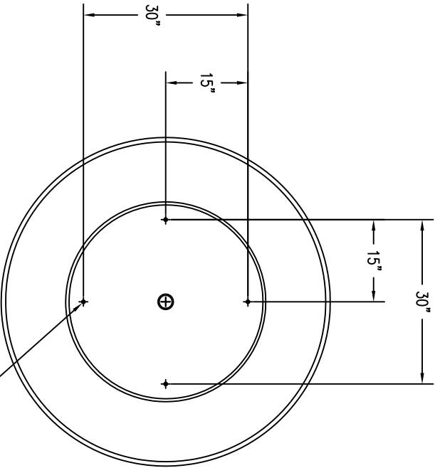
4 CROSS SECTION
