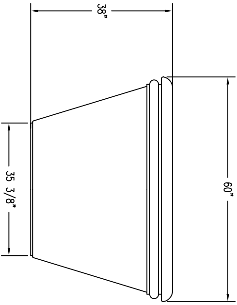
2 ELEVATION VIEW
