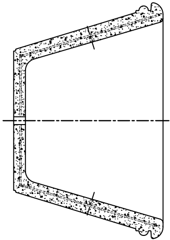
4 CROSS SECTION
