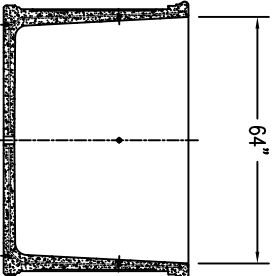
4 CROSS SECTION
