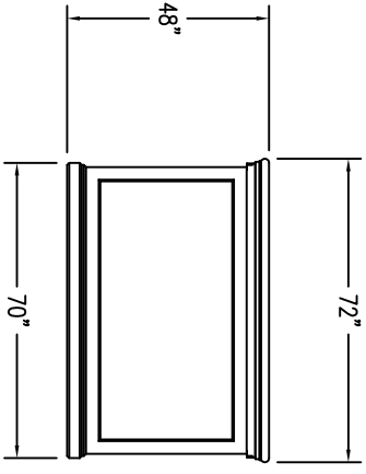
2 ELEVATION VIEW
