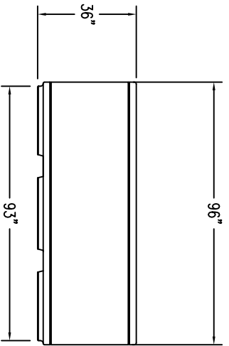
2 ELEVATION VIEW
