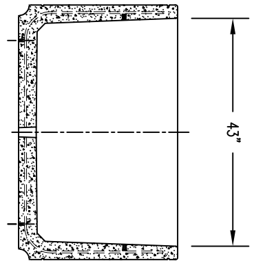
4 CROSS SECTION
