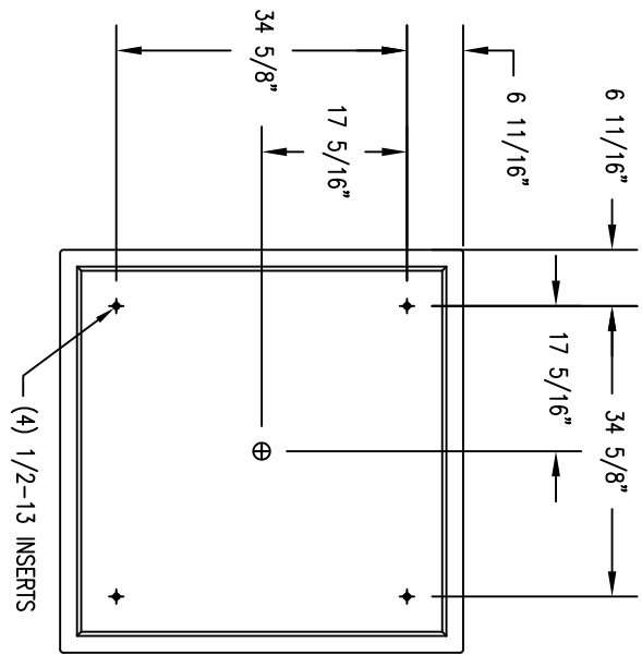
3 BOTTOM VIEW
