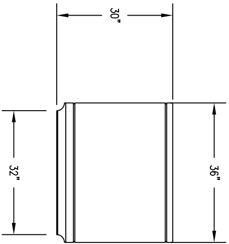
2 ELEVATION VIEW
