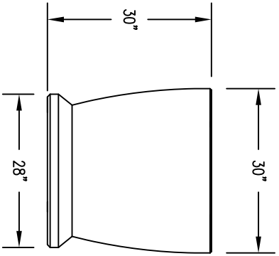
2 ELEVATION VIEW
