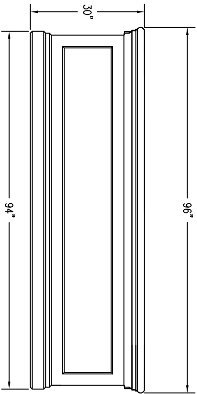
2 ELEVATION VIEW
