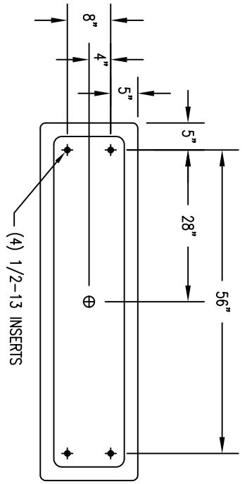
4 CROSS SECTION
