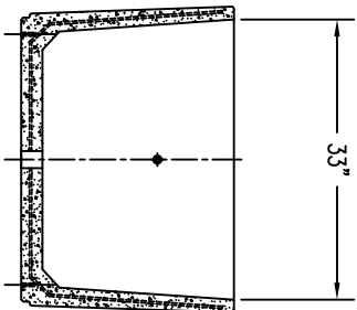
4 CROSS SECTION
