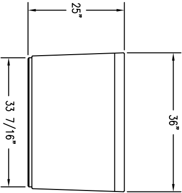
2 ELEVATION VIEW
