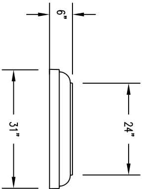
2 ELEVATION VIEW
