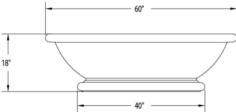
ELEVATION VIEW
