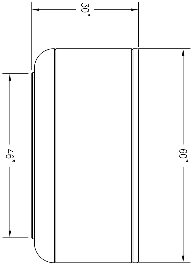
1 TOP VIEW
