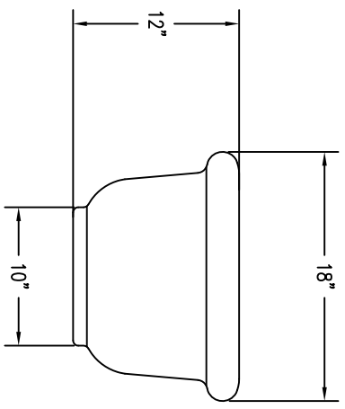
2 ELEVATION VIEW
