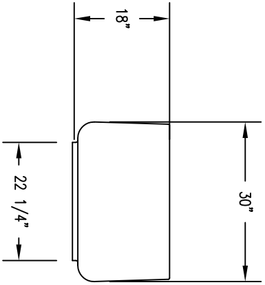
2 ELEVATION VIEW
