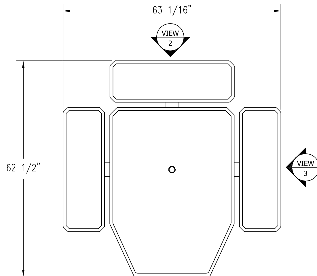
1 TOP VIEW Scale: 1/16" = 1"
