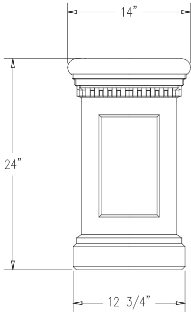
ELEVATION VIEW
