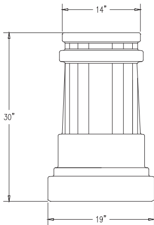
ELEVATION VIEW
