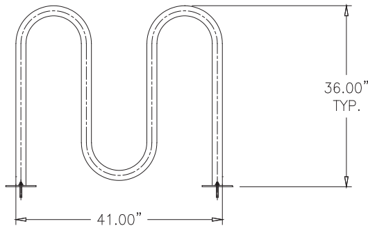
ELEVATION VIEW
