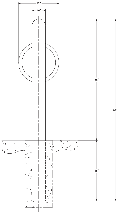
ELEVATION VIEW
