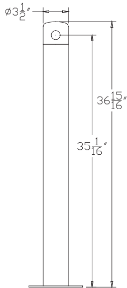
ELEVATION VIEW
