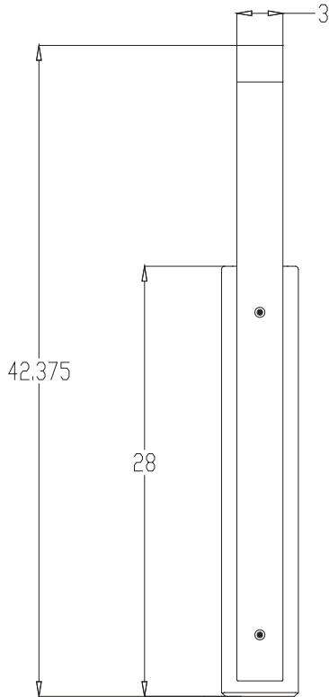
ELEVATION VIEW
