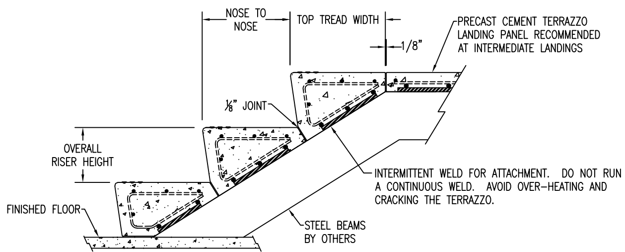
2 PARTIAL STAIR SECTION SS-51 TREAD Scale: 1 1/2" = 1'
