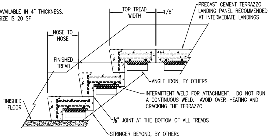
2 PARTIAL STAIR SECTION SS-31 T/R Scale: 1 1/2" = 1'
