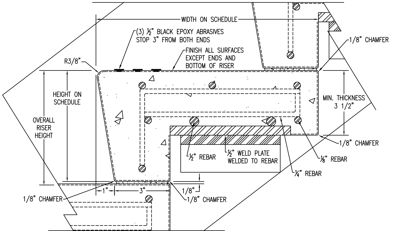
1 SECTION OF SS-31 TREAD Scale: 6" = 1'-0"
