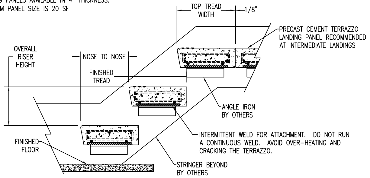
2 PARTIAL STAIR SECTION SS-30 TREAD Scale: 1 1/2" = 1'
