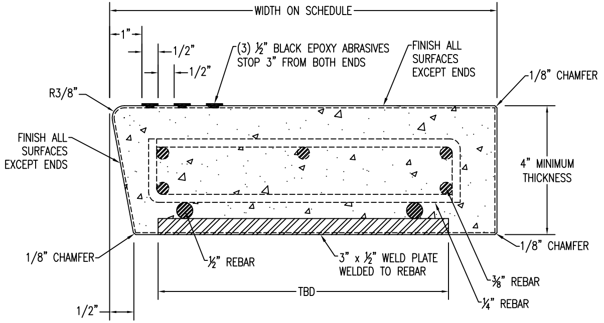
1 SECTION OF SS-30 TREAD Scale: 6" = 1'-0"
