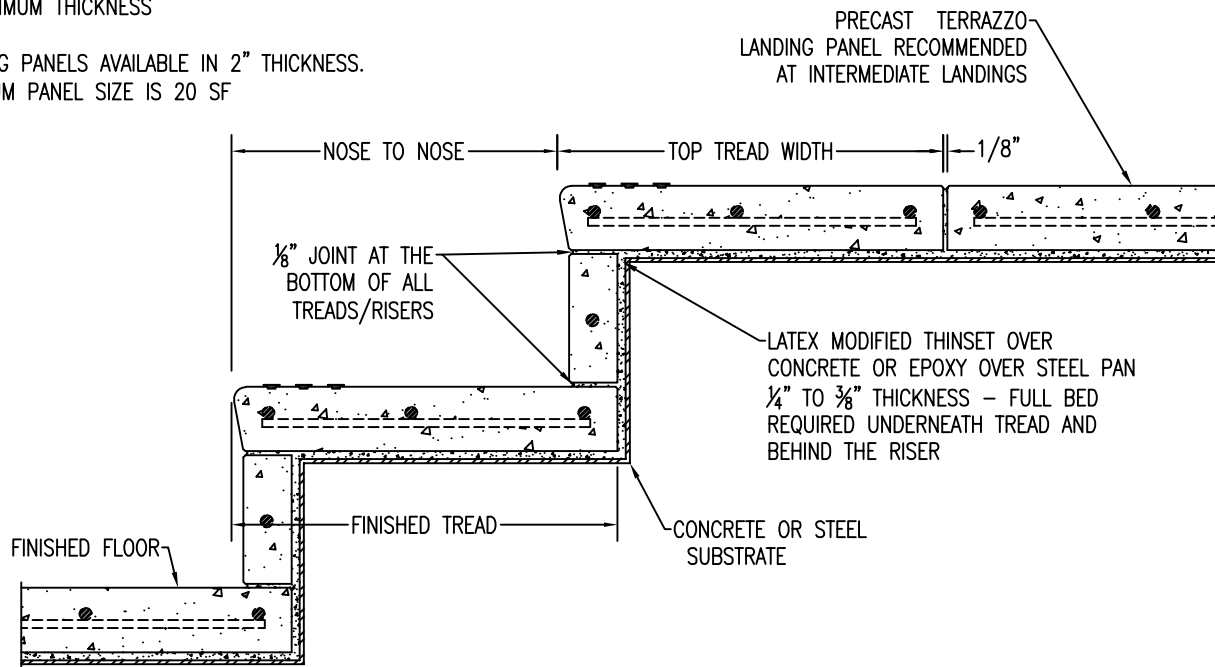
2 PARTIAL STAIR SECTION S-40 T/R Scale: 3" = 1'
