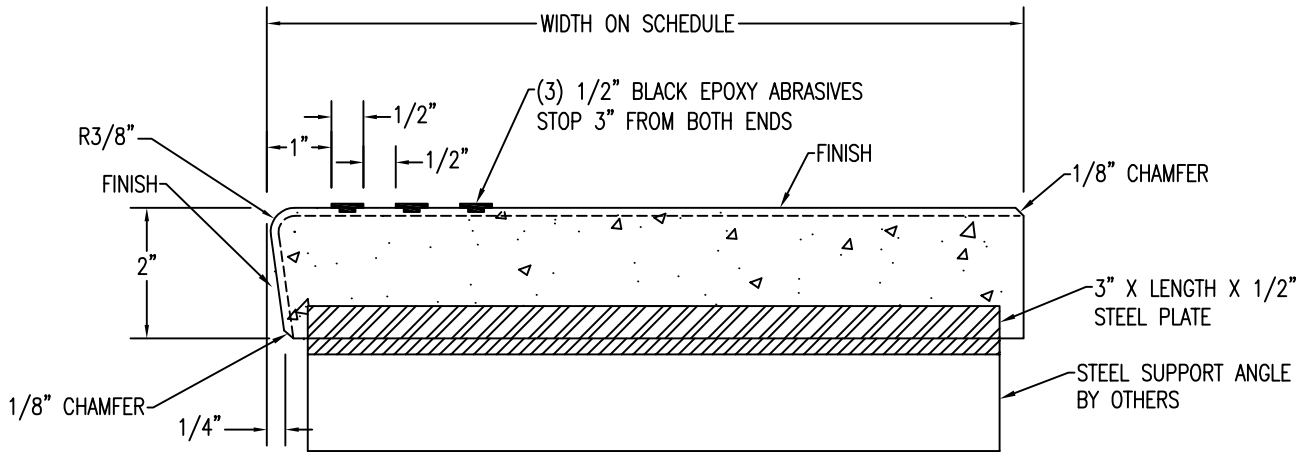
1 SECTION VIEW ESS-30 TREAD Scale: 6" = 1'-0"
