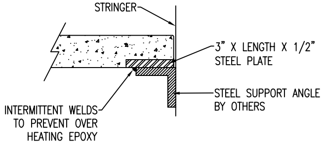
2 ELEVATION SECTION ESS-30 TREAD Scale: 6" = 1'-0"
