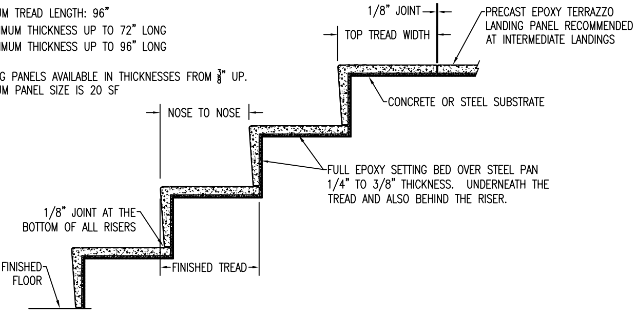
2 PARTIAL STAIR SECTION E-31 T/R Scale: 3" = 1'
