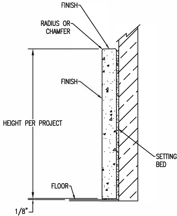
2 SECTION VIEW WALL PANEL Scale: FULL
