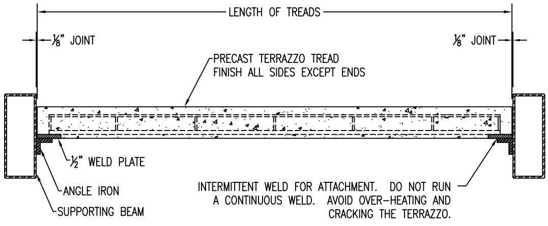
2 SECTION FRONT VIEW ANGLE IRON Scale: 1 1/2" = 1'-0"
