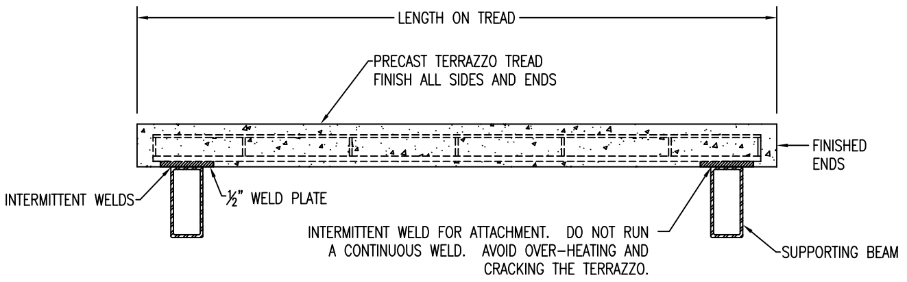
1 SECTION FRONT VIEW SUPPORTING BEAM Scale: 1 1/2" = 1'-0"
