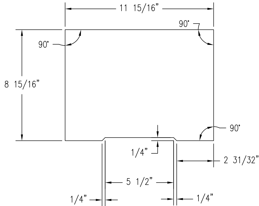
1 PAVER - PLAN VIEW
